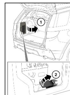
Land Rover Discovery Sport (L550)
