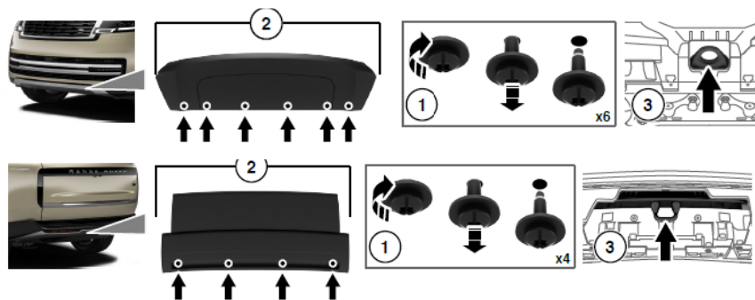
Front and rear towing location examples, Range Rover (L460)
