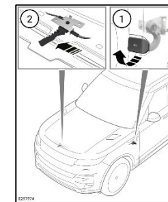
Hood lever locations example – Range Rover Sport (L461) LHD
