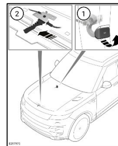
Hood lever locations example – Range Rover Sport (L461) RHD
